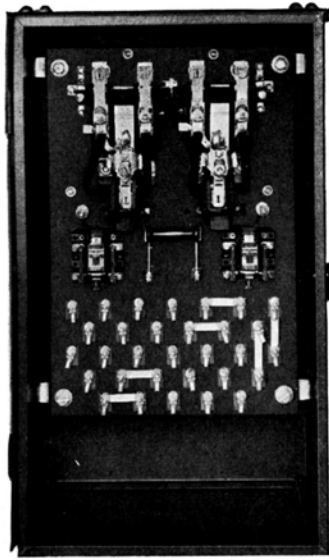
FIGURE 37. The motor control panel.
