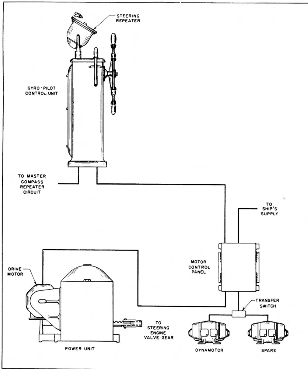
FIGURE 34. Gyro-Pilot arrangement.
