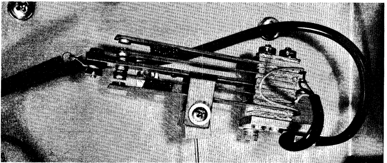
Figure 5-12. Servo Contactor
