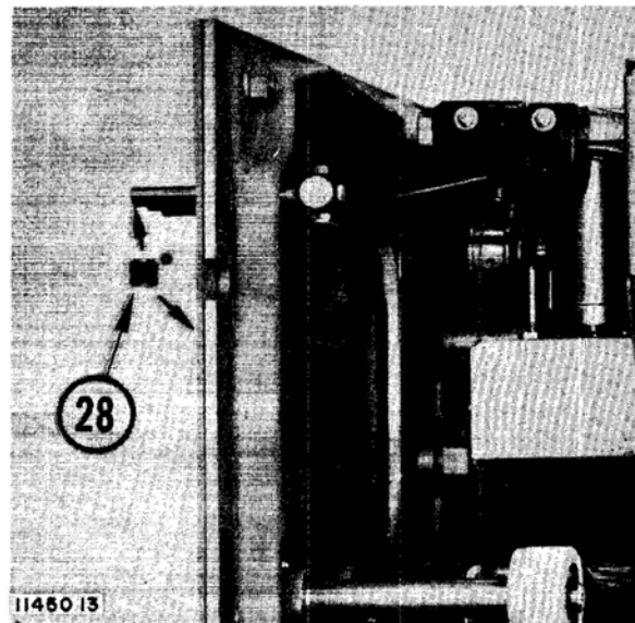
Figure 5-19e. Tension Arm Assembly Removal and Replacement
