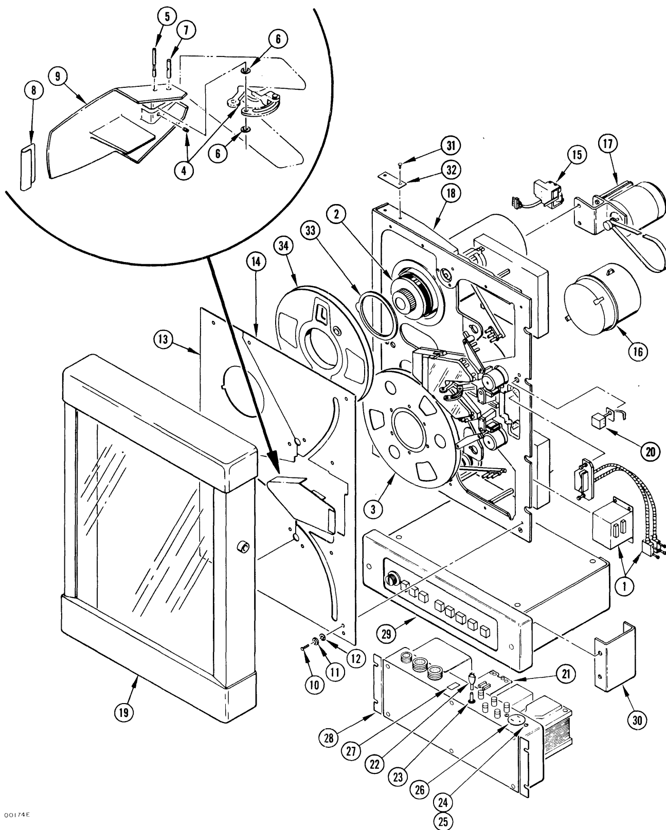
Figure 7-1. SDSTM-407 Tape Transport
