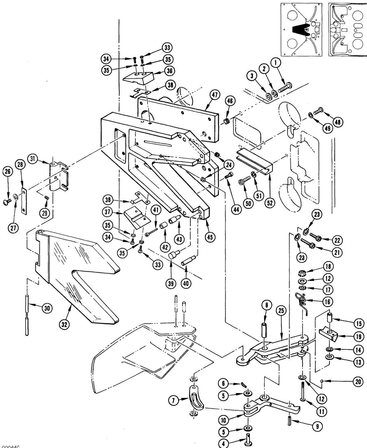
Figure 7-8. Vacuum Chamber
