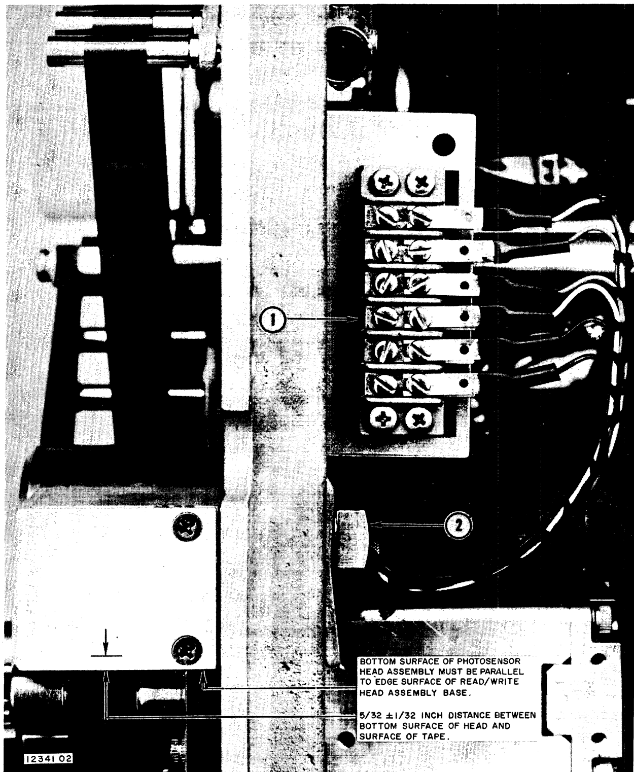
Figure 5-23. Photosensor Head Assembly Removal and Replacement
