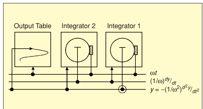
Figure 3. Schematic setup for simple harmonic motion. The notation used is that of Bush [1] and is largely self explanatory. Bus shafts are labeled according to the quantities they represent.
