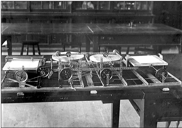
Figure 11. A delightfully simple model. This model, built by 15-year-old “Digby” Worthy around 1939, is remarkable for its simplicity. A system of belts and pulleys replaces the conventional geared interconnect, allowing the system to be constructed with a mere handful of parts. (Courtesy of P. Worthy.)
