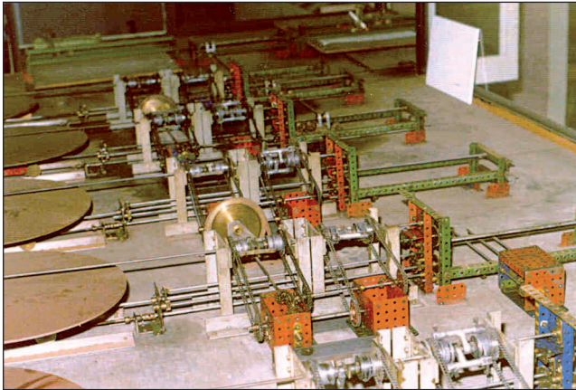
Figure 9. The Cambridge model on display at MOTAT in 1978. Integrator disks can be seen on the left. The torque amplifiers, powered through chain drives, are down the center. Just visible at the rear are the input and output tables. (Courtesy of A. Barton.)
