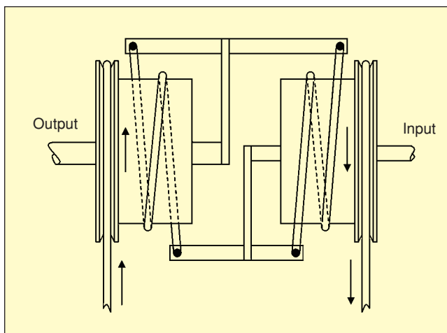
Figure 4. Principle of the torque amplifier. Two drums are continuously rotated in opposite directions by an electric motor. When the input shaft turns, one of the bands is tightened around its drum, while the other is slackened, causing the output shaft to be turned in the same direction as the input but with much greater torque.
