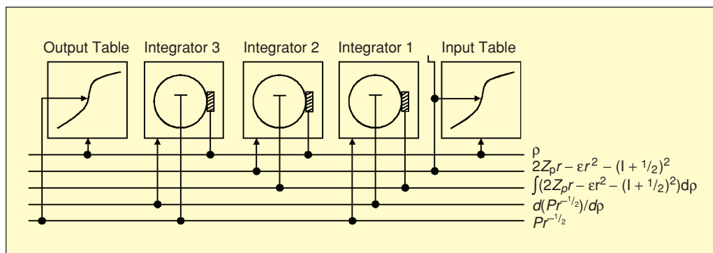
Figure 6. Schematic setup for the chromium atom wavefunction. The equation being solved by this setup is d/d\rho(Pr^{-1/2}) = -\int(2Z\rho r - \epsilon r^2 - (l + 1/2)^2)Pr^{-1/2}d\rho , where \rho = \log r . The output table records the value of Pr^{-1/2} as a function of \log r .
