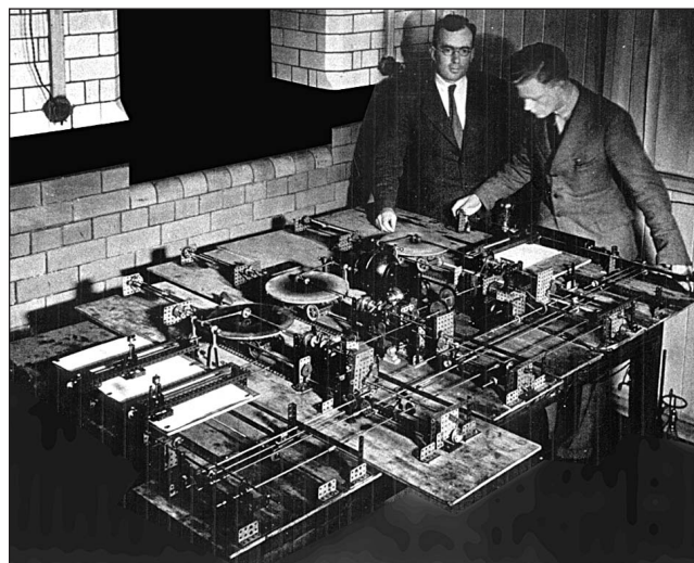
Figure 5. Hartree and Porter with the Meccano model. The three integrators are in the center of the machine. The motor powering the torque amplifiers can be seen between them. On the left is the dual-output table, and on the right is an input table being operated by Porter. (Courtesy of R. Hartree.)
