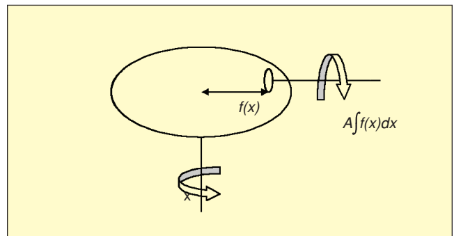
Figure 2. Wheel and disk integrator. The displacement of the wheel from the center of the disk, which is continuously variable, represents the function f(x) . The position of the shaft carrying the disk represents the value of the variable x . The motion of the shaft carrying the wheel is then proportional to the required integral.
