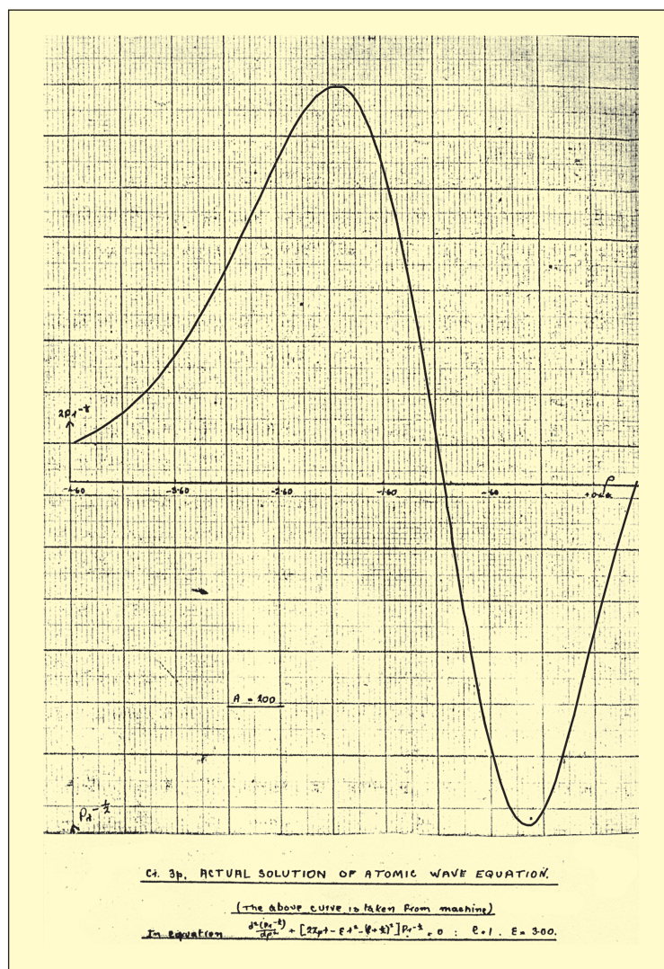
Figure 7. Actual output from the Meccano model. This plot is taken from the M.S. thesis of A. Porter, which, along with a single integrator from his model, now forms part of a permanent display at the Science Museum in London. (Courtesy of A. Porter.)
