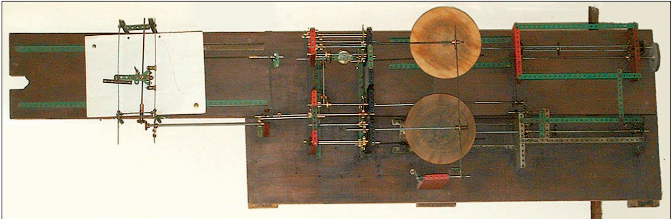
Figure 10. Demonstration model of N. Eyres. This model was recently rediscovered with plotted output still attached to the output table. It is now being restored by Mr Eyres' son-in-law, who kindly provided the photograph. (Courtesy of D. Fargus.)
