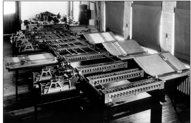
Figure 1. Vannevar Bush's prototype differential analyzer at MIT in 1931. On the left are the six integrators in pairs, with the output table between them. On the right are four input tables. Down the center runs the system of shafts, which could be reconfigured to interconnect the units for a specific problem. (Courtesy of the MIT Museum.)
